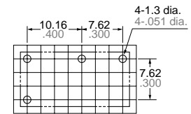
PC board pattern (Copper-side view)
