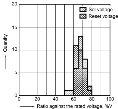
8. Distribution of set and reset voltage
