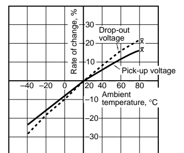
9. Ambient temperature characteristics
