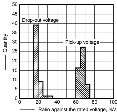
7. Distribution of pick-up and drop-out voltage
