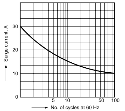
2-1. Surge current and time (OAC)
