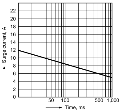
2-2. Surge current and time (IDC)
