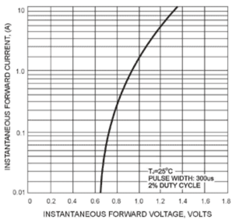
FIG. 4 - TYPICAL FORWARD CHARACTERISTICS
