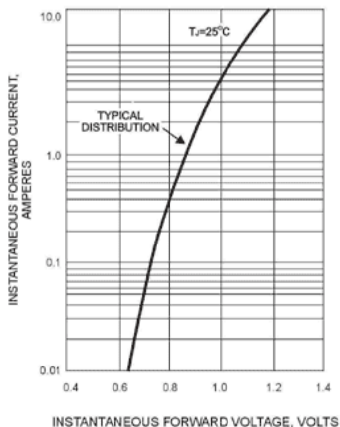
FIG. 3 - TYPICAL FORWARD CHARACTERISTICS
