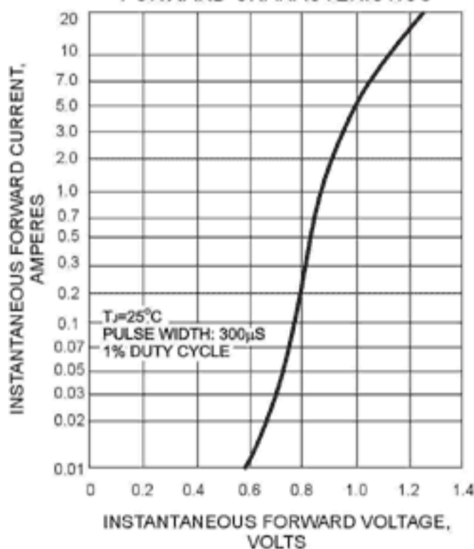
FIG. 4 - TYPICAL INSTANTANEOUS FORWARD CHARACTERISTICS
