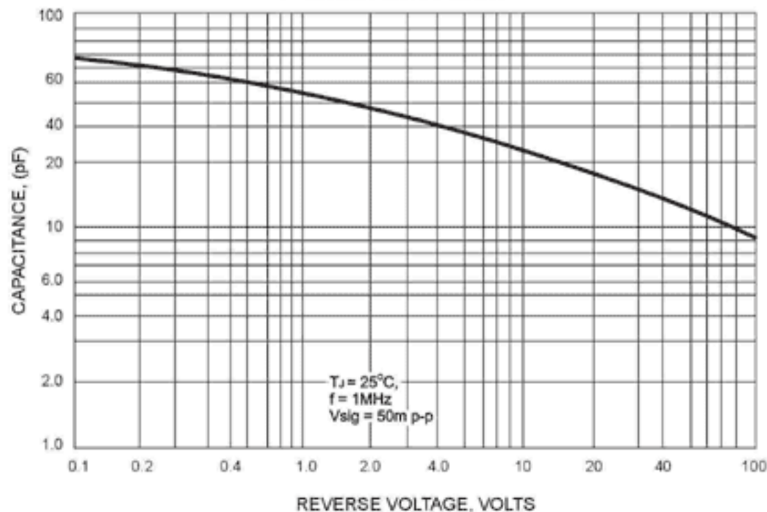
FIG. 5 - TYPICAL JUNCTION CAPACITANCE PER BRIDGE ELEMENT
