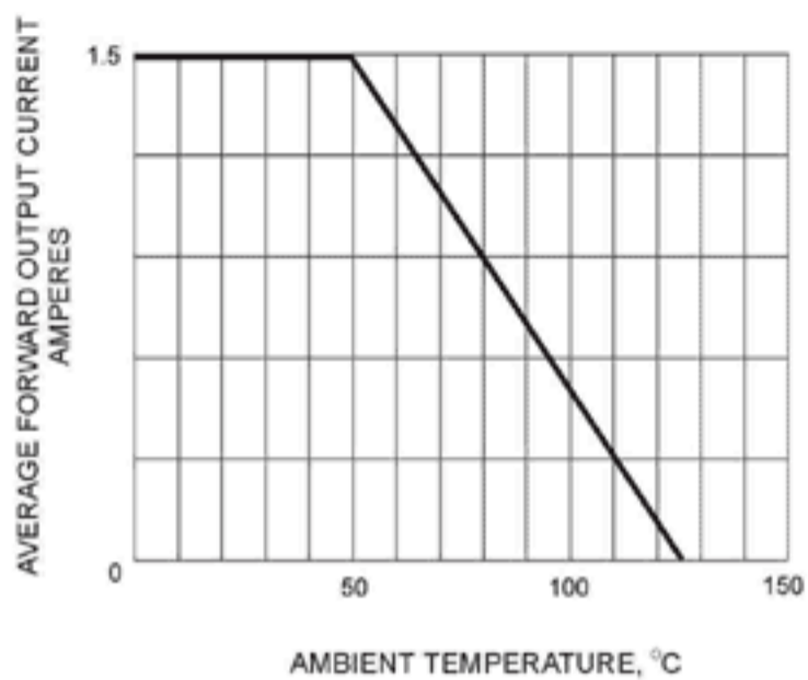
FIG. 1 - DERATING CURVE OUTPUT RECTIFIED CURRENT
