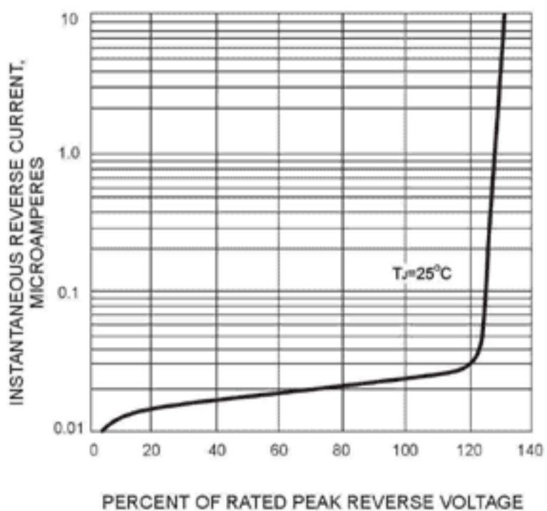
FIG. 3 - TYPICAL REVERSE CHARACTERISTICS
