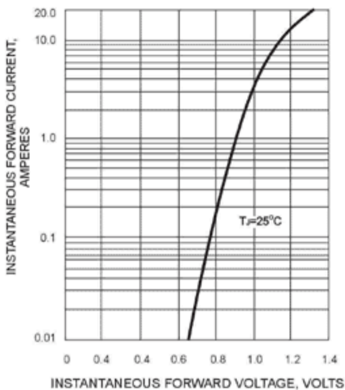
FIG. 2 - TYPICAL FORWARD CHARACTERISTICS
