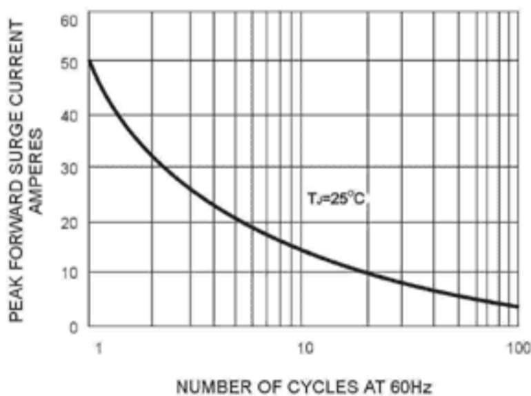
FIG. 4 - MAXIMUM FORWARD SURGE CURRENT
