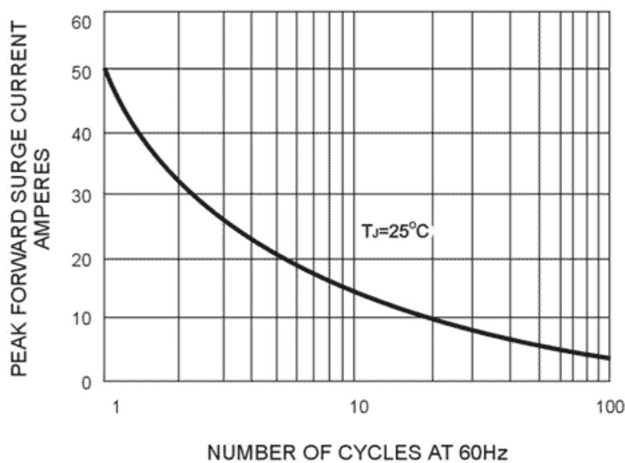
FIG. 4 - MAXIMUM FORWARD SURGE CURRENT
