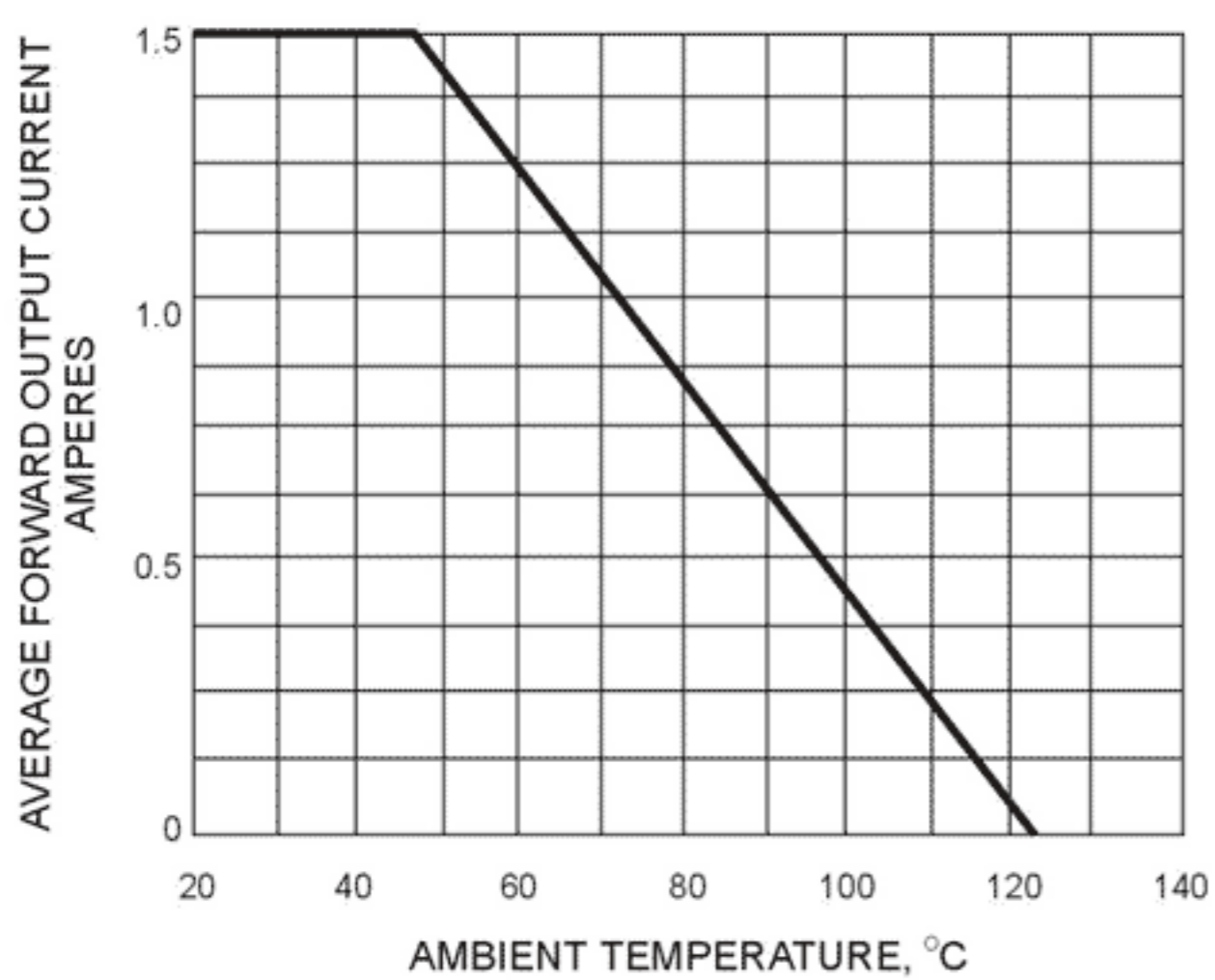
FIG. 1 - DERATING CURVE OUTPUT RECTIFIED CURRENT
