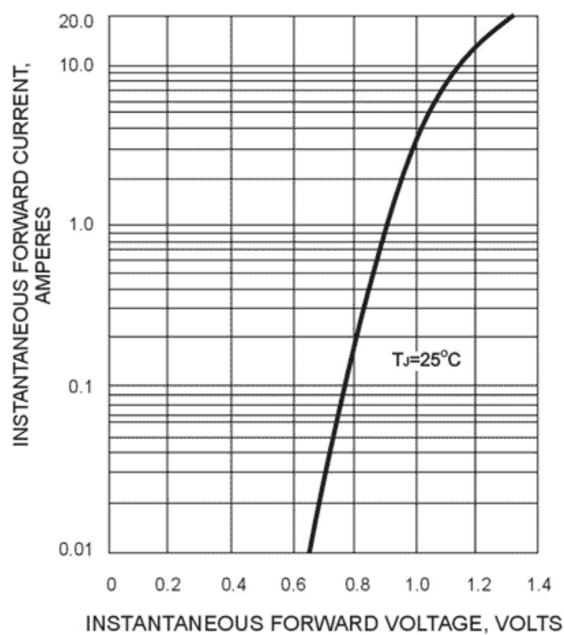
FIG. 2 - TYPICAL FORWARD CHARACTERISTICS
