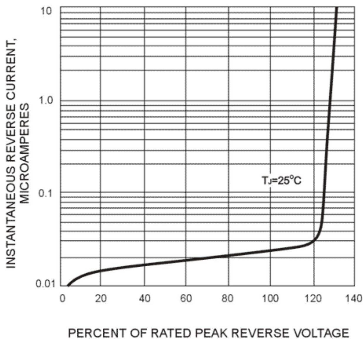
FIG. 3 - TYPICAL REVERSE CHARACTERISTICS
