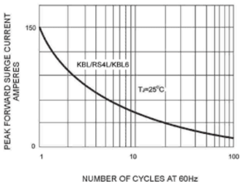
FIG. 1 - MAXIMUM FORWARD SURGE CURRENT
