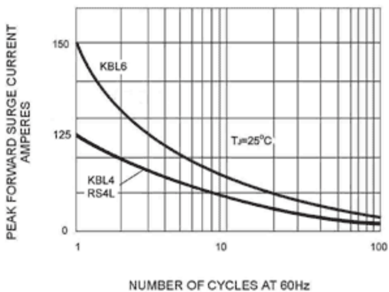
FIG. 1 - MAXIMUM FORWARD SURGE CURRENT
