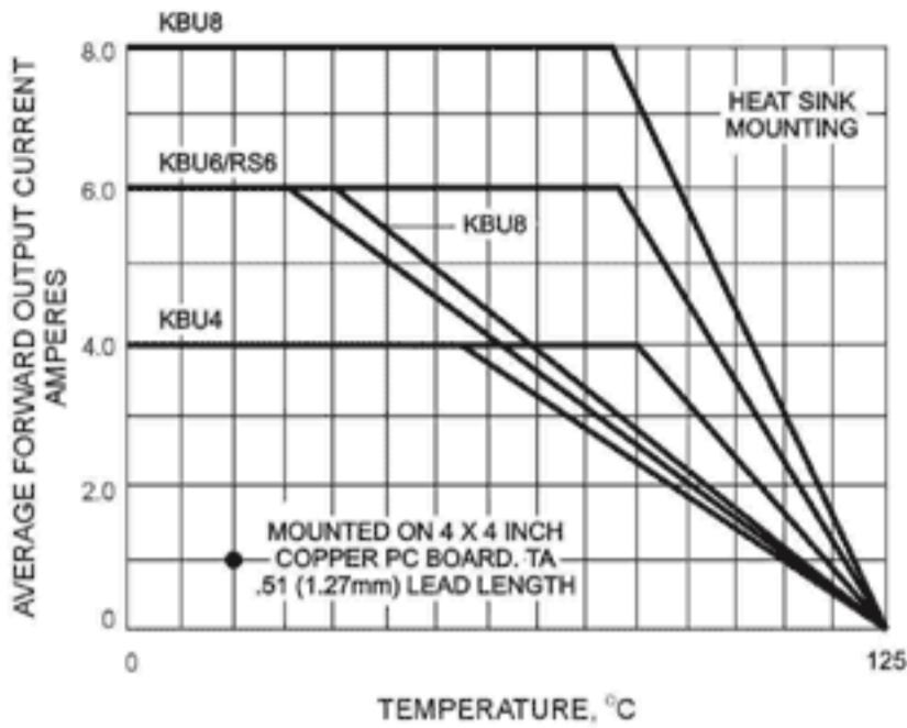
FIG. 1 - DERATING CURVE FOR OUTPUT RECTIFIED CURRENT
