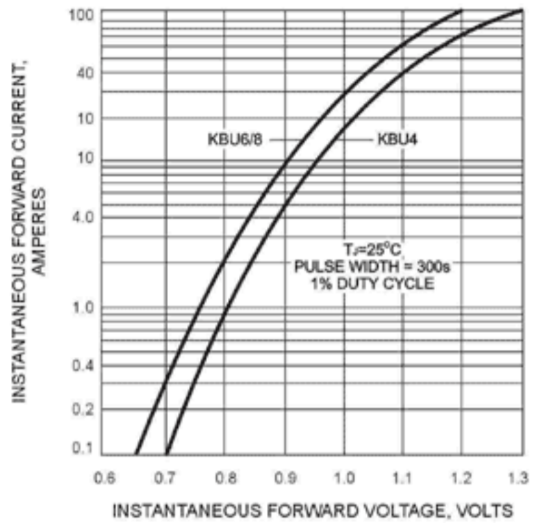
FIG. 2 - TYPICAL INSTANTANEOUS FORWARD CHARACTERISTIC
