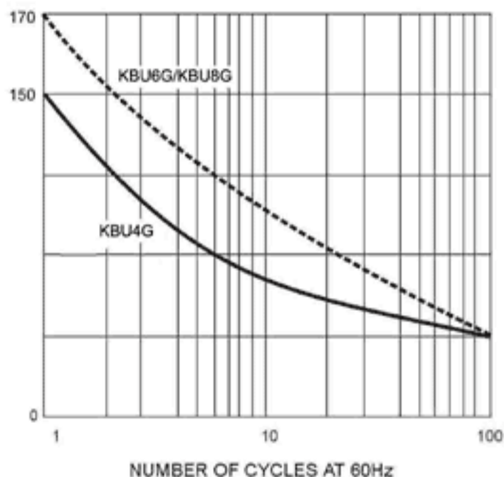
FIG. 3 - MAXIMUM NON-RETETITIVE PEAK FORWARD SURGE CURRENT
