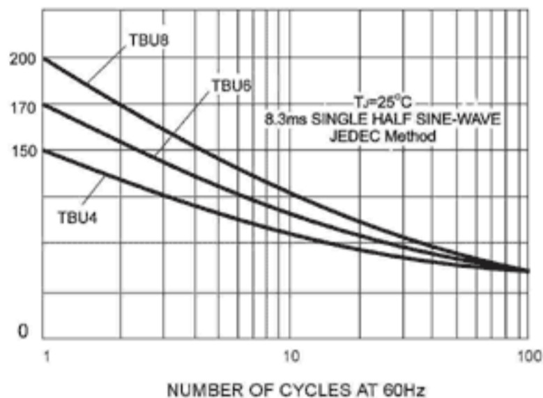
FIG. 3 - MAXIMUM NON-RETRITIVE PEAK FORWARD SURGE CURRENT
