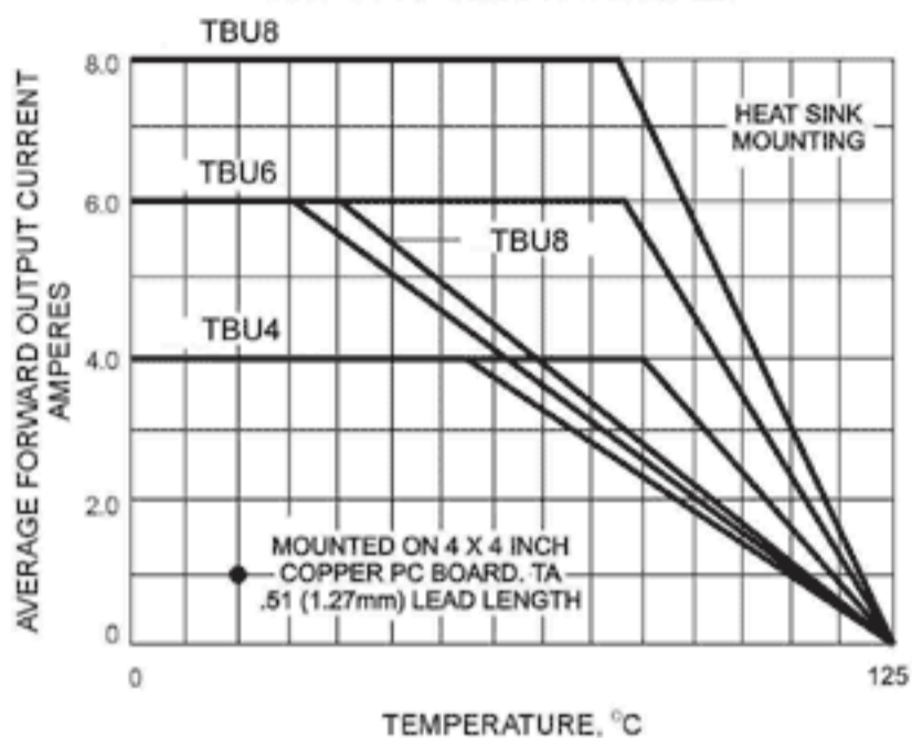
FIG. 1 - DERATING CURVE FOR OUTPUT RECTIFIED CURRENT
