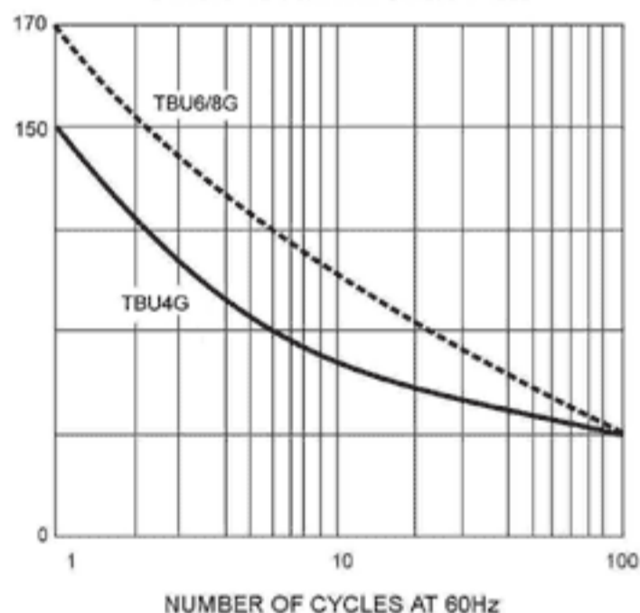
FIG. 3 - MAXIMUM NON-RETRITIVE PEAK FORWARD SURGE CURRENT
