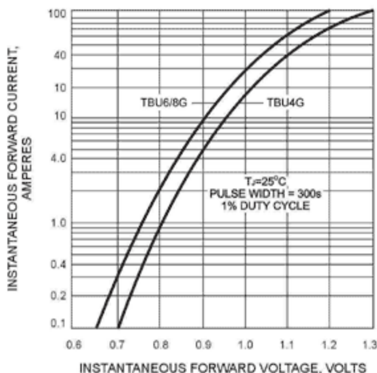
FIG. 2 - TYPICAL INSTANTANEOUS FORWARD CHARACTERISTIC
