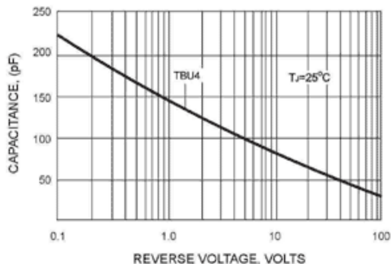
FIG. 5 - TYPICAL JUNCTION CAPACITANCE PER ELEMENT
