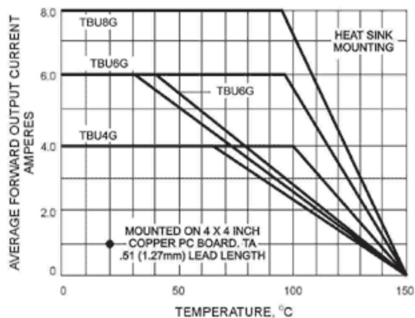
FIG. 1 - DERATING CURVE FOR OUTPUT RECTIFIED CURRENT
