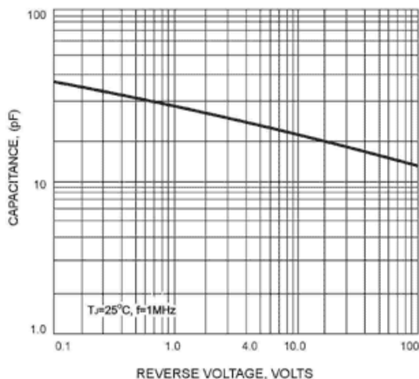
FIG. 3 - TYPICAL JUNCTION CAPACITANCE
