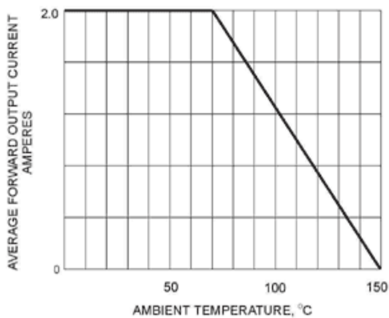
FIG. 1 - DERATING CURVE OUTPUT RECTIFIED CURRENT
