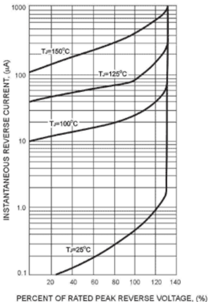
FIG. 5 - TYPICAL REVERSE CHARACTERISTICS
