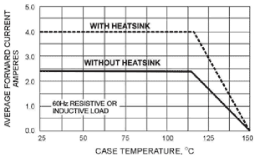
FIG. 1 - FORWARD CURRENT DERATING CURVE
