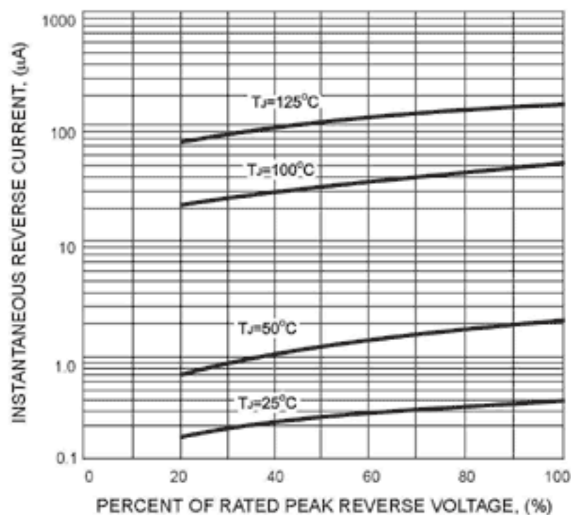
FIG. 5 - TYPICAL REVERSE CHARACTERISTICS
