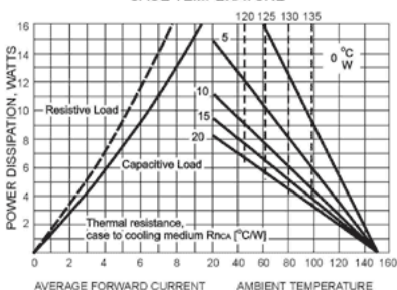
FIG. 6 - MEAN AVERAGE FORWARD CURRENT CASE TEMPERATURE
