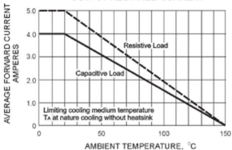
FIG. 1 - DERATING CURVE FOR OUTPUT RECTIFIED CURRENT
