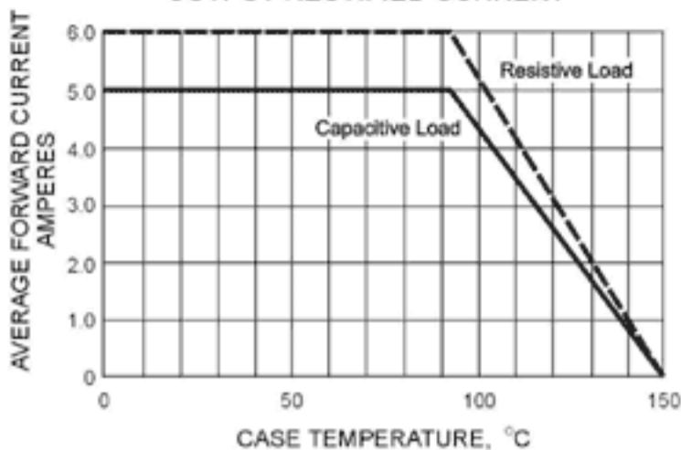
FIG. 2 - DERATING CURVE FOR OUTPUT RECTIFIED CURRENT
