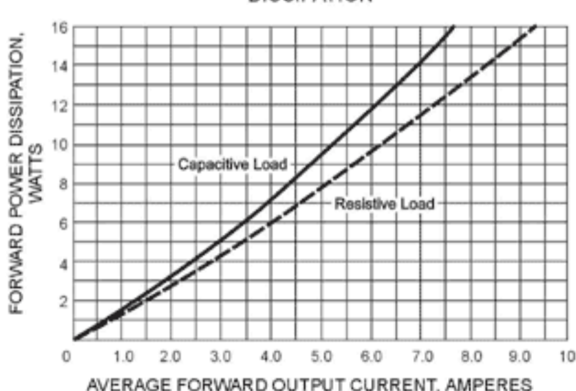
FIG. 5 - MAXIMUM TOTAL BRIDGE POWER DISSIPATION
