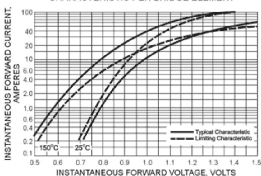
FIG. 3 - TYPICAL INSTANTANEOUS FORWARD CHARACTERISTIC PER BRIDGE ELEMENT
