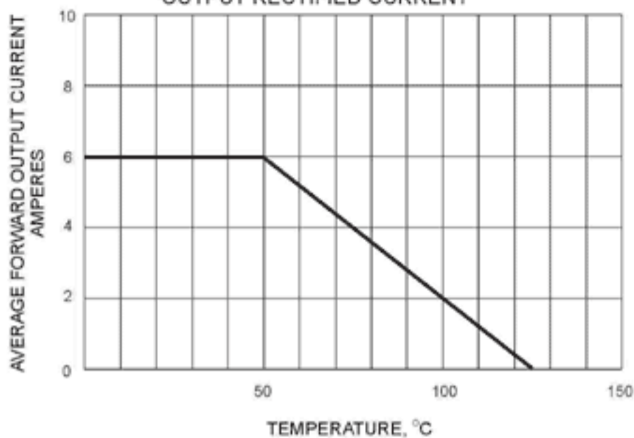
FIG. 1 - DERATING CURVE FOR OUTPUT RECTIFIED CURRENT
