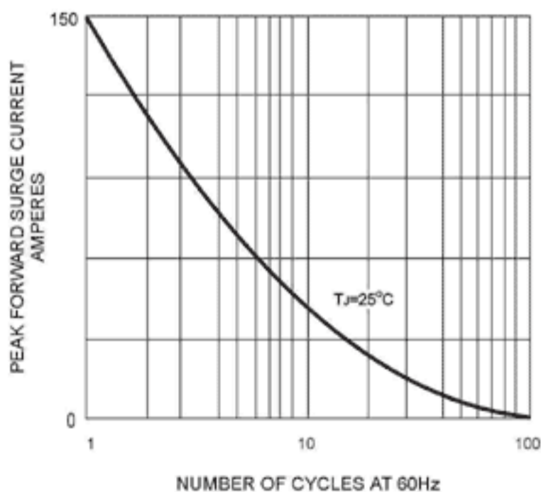
FIG. 3 - MAXIMUM FORWARD SURGE CURRENT
