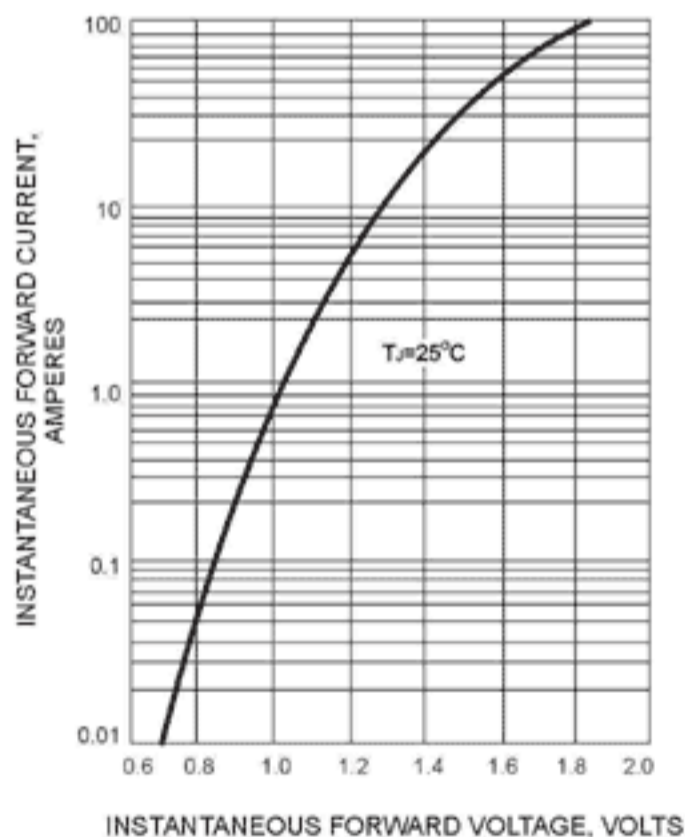
FIG. 4 - TYPICAL INSTANTANEOUS FORWARD CHARACTERISTICS
