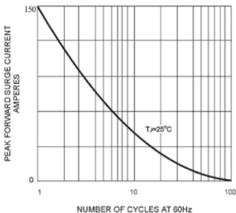
FIG. 3 - MAXIMUM FORWARD SURGE CURRENT
