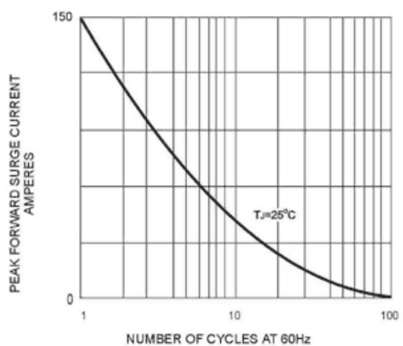
FIG. 1 - MAXIMUM FORWARD SURGE CURRENT
