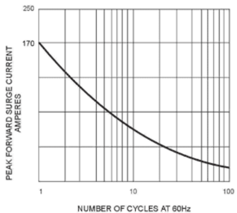
FIG. 1 - MAXIMUM FORWARD SURGE CURRENT
