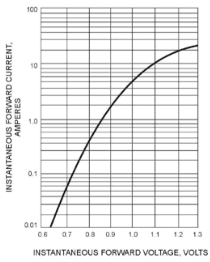
FIG. 3 - TYPICAL FORWARD CHARACTERISTICS
