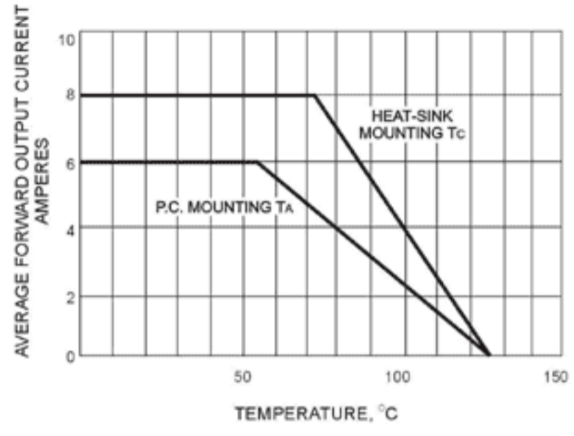
FIG. 2 - DERATING CURVE OUTPUT RECTIFIED CURRENT
