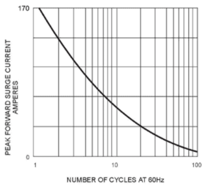
FIG. 1 - MAXIMUM FORWARD SURGE CURRENT
