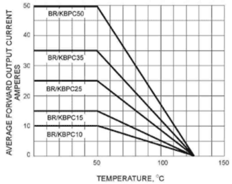
FIG. 2 - DERATING CURVE OUTPUT RECTIFIED CURRENT
