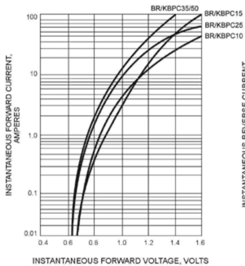
FIG. 3 - TYPICAL FORWARD CHARACTERISTICS
