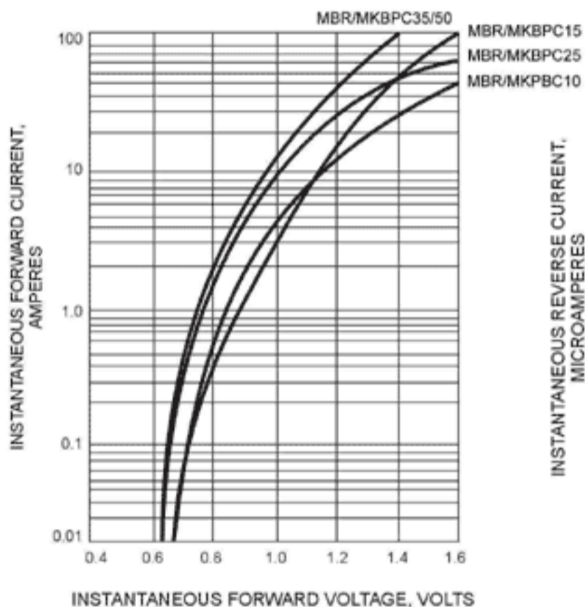
FIG. 3 - TYPICAL FORWARD CHARACTERISTICS
