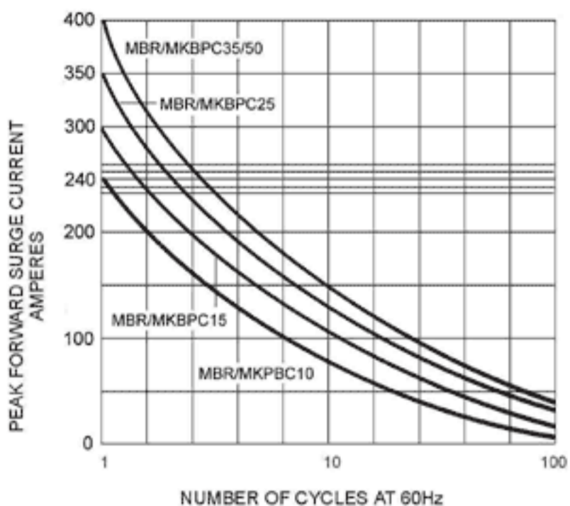
FIG. 1 - MAXIMUM FORWARD SURGE CURRENT
