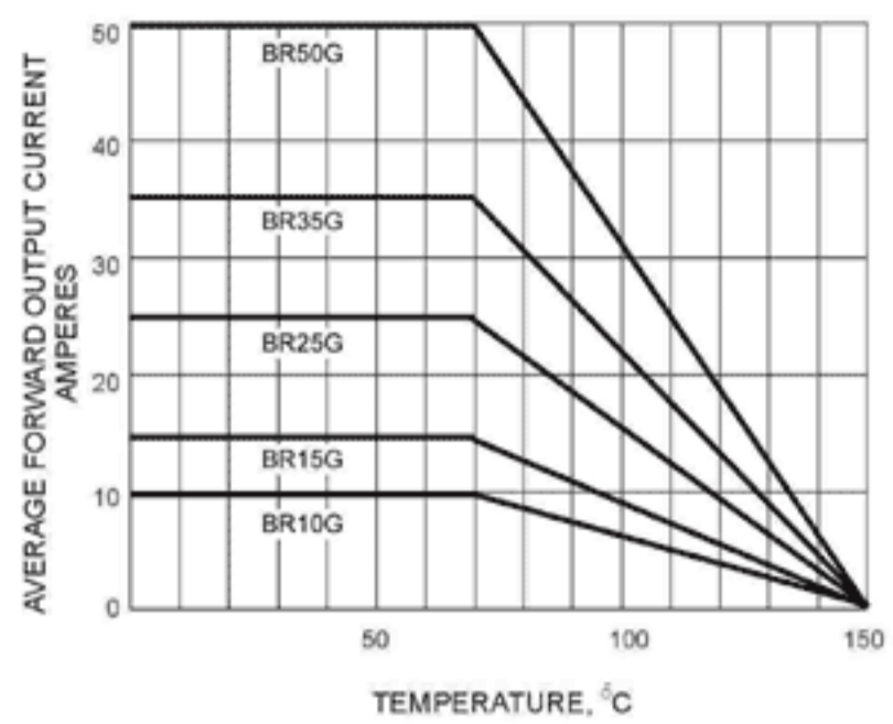
FIG. 2 - DERATING CURVE OUTPUT RECTIFIED CURRENT
