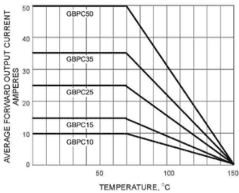
FIG. 2 - DERATING CURVE OUTPUT RECTIFIED CURRENT
