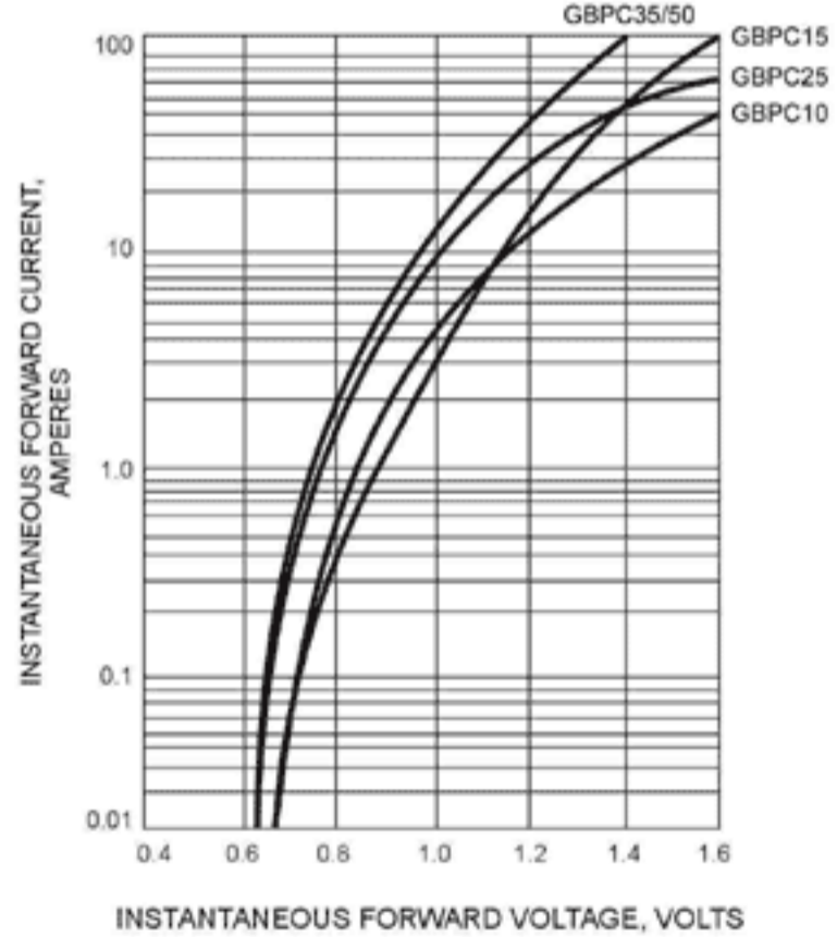
FIG. 3 - TYPICAL FORWARD CHARACTERISTICS
