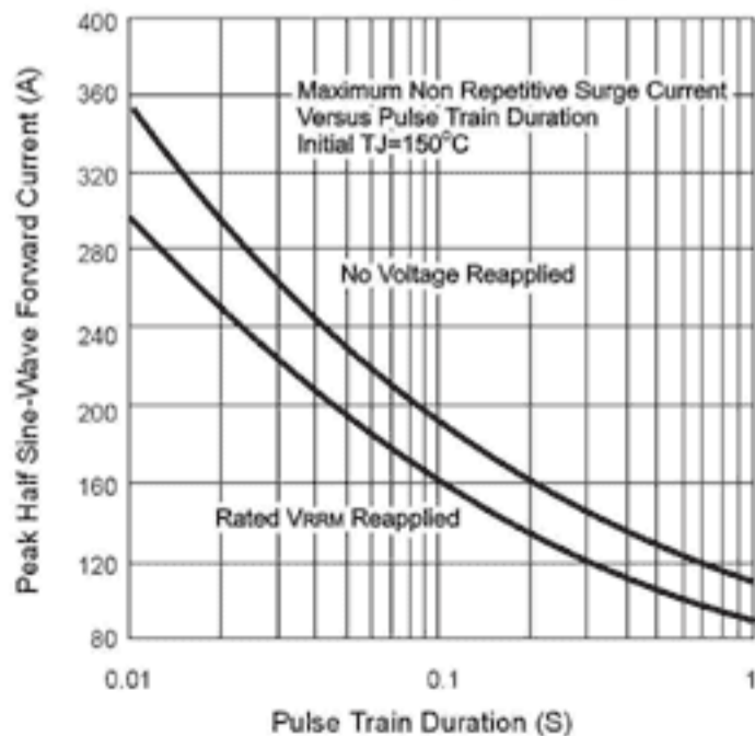
FIG. 5 - Maximum Non-Repetitive Surge Current
