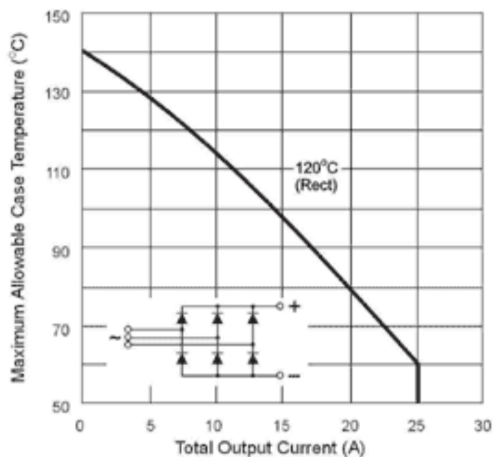
FIG. 1 - Current Rating Characteristics
