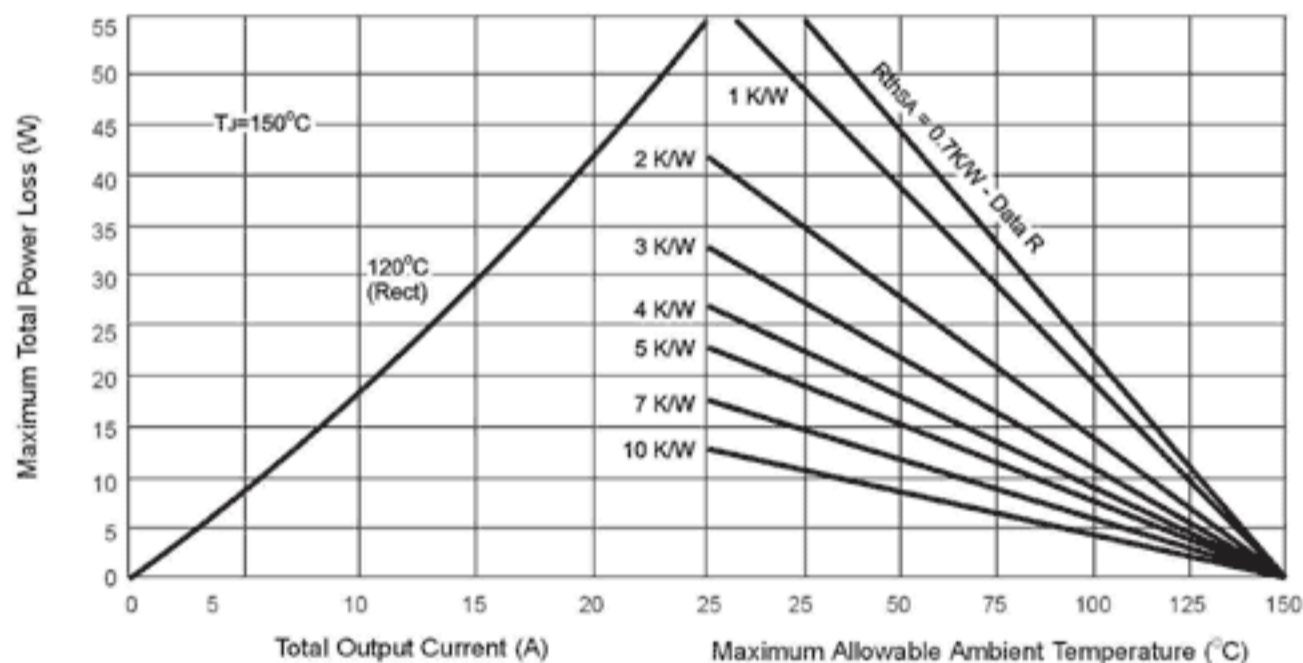
FIG. 3 - Total Power Loss Characteristics
