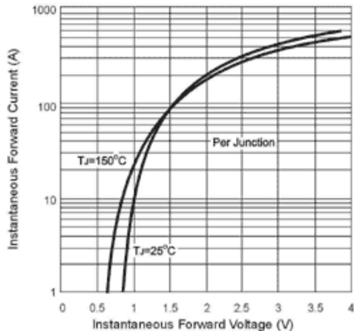
FIG. 2 - Forward Voltage Drop Characteristics
