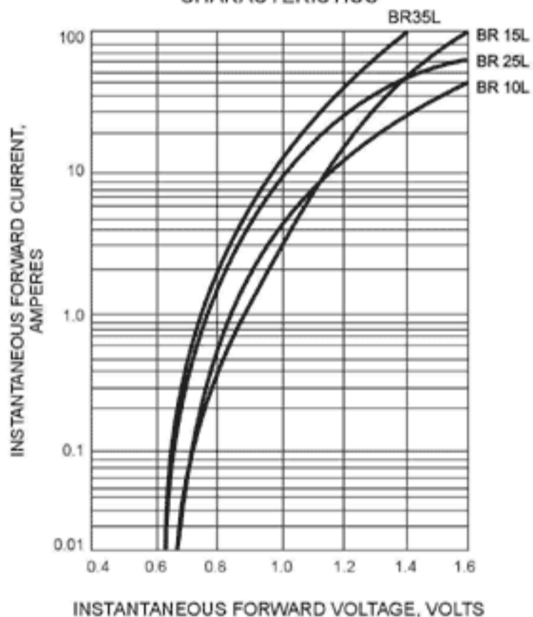
FIG. 3 - TYPICAL FORWARD CHARACTERISTICS
