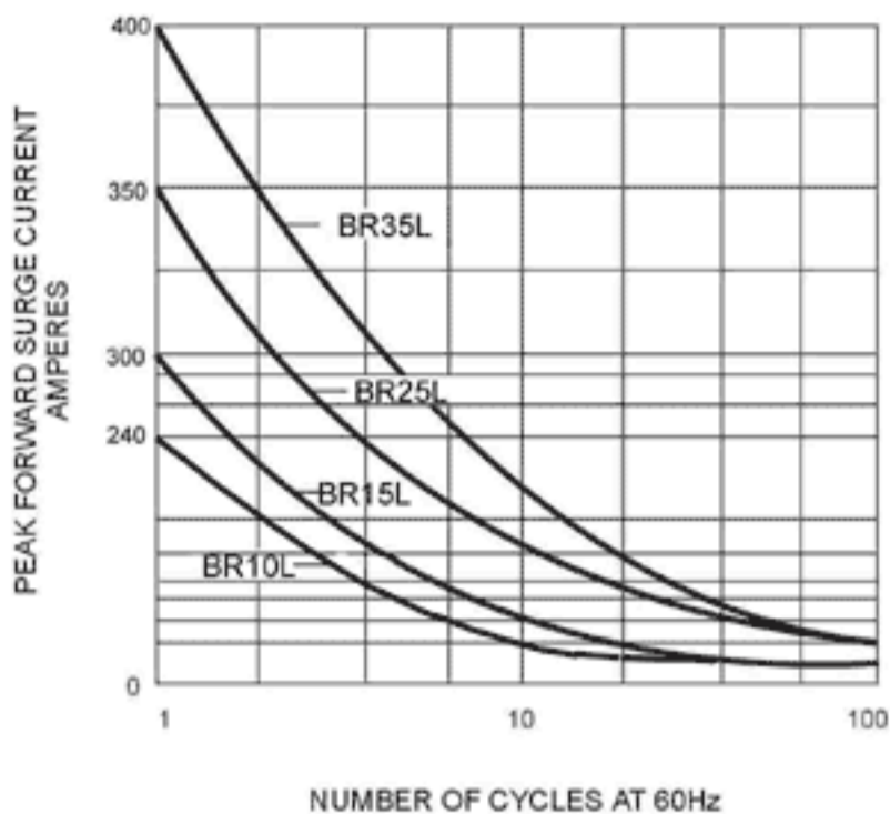
FIG. 1 - MAXIMUM FORWARD SURGE CURRENT
